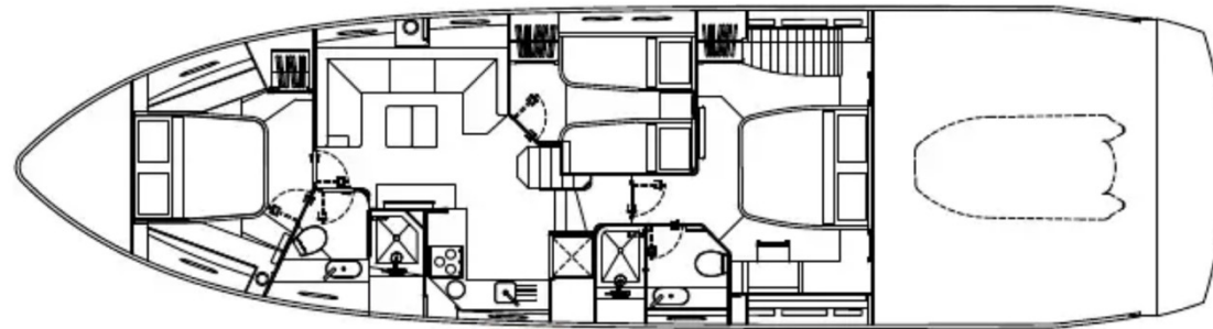
Lower deck Shown with tender size to suit open cockpit arrangement
